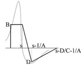
Fig. 4. X_{post} as piecewise linear function Eq. (14). The action potential represented by this X_{post} is outlined in gray in the background.
