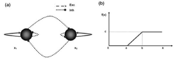
Fig. 1. a) The recurrent competitive two-node network has self-excitatory connections that help store a pattern in WM, and inhibitory connections within and between units. b) The piecewise activation function f(x) .
