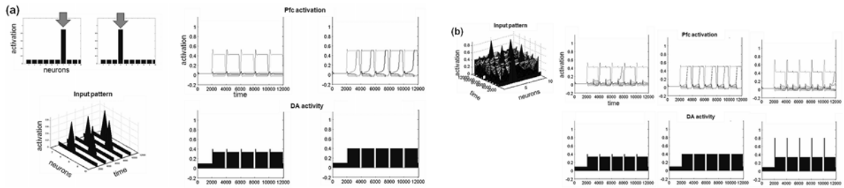
Fig. 4. Activation traces represent the activation of different excitatory neurons. a) sWM task. The input pattern (top, left) is presented to the Pfc network for 2000 msec. The top rows show the activation of the pyramidal neuron x over for variable levels of DAergic activity (bottom row). Notice how DA regulates the storage of activation in WM, as well as the formation of a spatial pattern in the Pfc field. Lack of DAergic activity prevents the storage of activation in WM, whereas a phasic DAergic input followed by a tonic baseline is optimal for WM storage. b) sWM task in the presence of noise. The input pattern is represented in the left inset. The 50-msec-noise interferes with the WM pattern that decays due to the absence of a tonic DA baseline (left panels). A hyperactive tonic DAergic input causes the loss of the pattern (middle panels). This effect is mainly due to the multiplicative effect of DA on self-excitation and to the intrinsic dynamics of the on-center/off-surround architecture. An initial phasic-tonic DAergic transmission prevents noise to disrupt the pattern (right panels).
