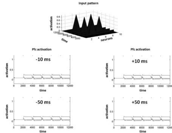
Figure 6. Effect of time jitter in the arrival of the DAergic input in Pfc during the DaAT task. A jitter of +/-10 ms and +/-50 ms in the DAergic spike with respect to the arrival time of the input produces no qualitative change in network behavior.
